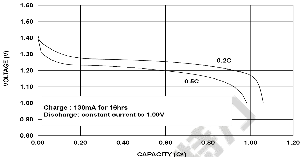
DISCHARGE CHARACTERISTICS OF BPI-48AA1300 CELL
