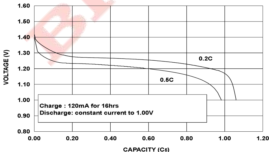
DISCHARGE CHARACTERISTICS OF BPI-48AA1200mAh CELL
