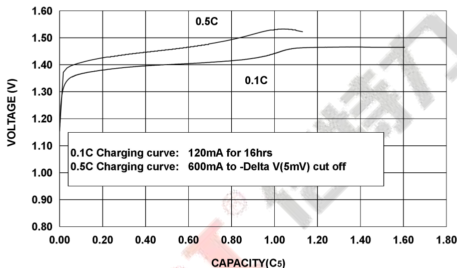
CHARGING CURVE OF BPI-48AA1200mAh CELL
