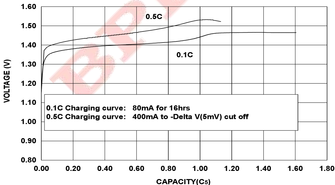
CHARGING CURVE OF BPI-44AAA800mAh CELL
