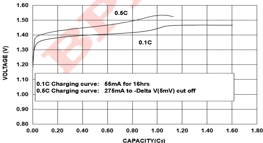
CHARGING CURVE OF BPI-43AAA550mAh CELL
