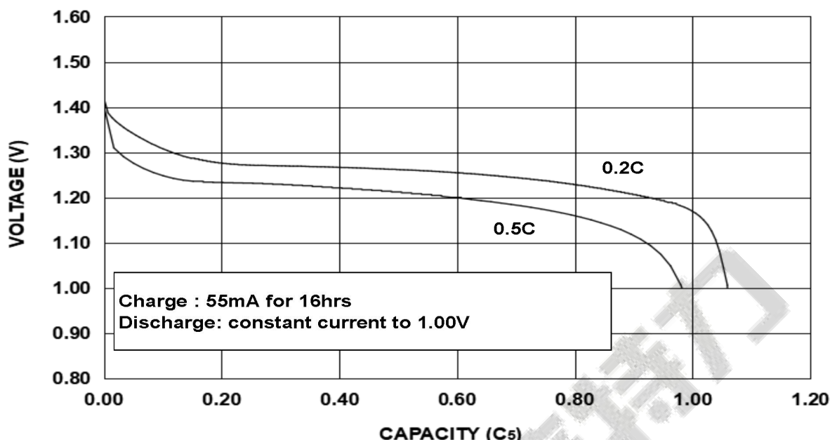
DISCHARGE CHARACTERISTICS OF BPI-43AAA550 mAh CELL
