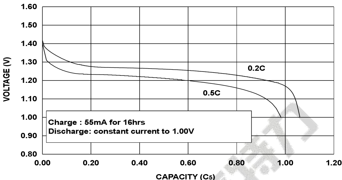
DISCHARGE CHARACTERISTICS OF BPI-43AAA500 mAh CELL
