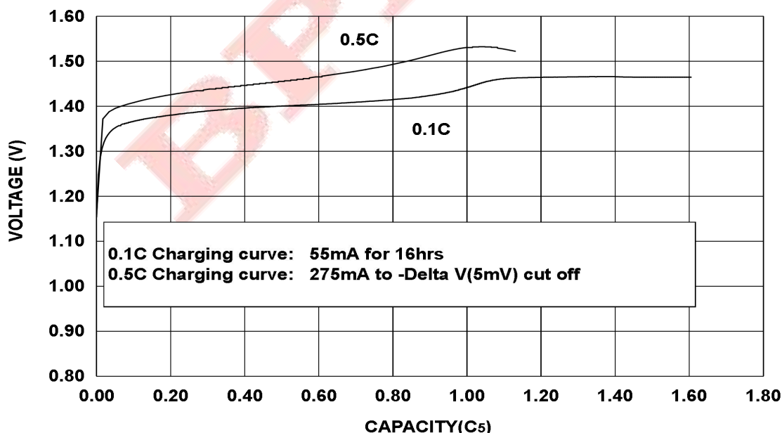
CHARGING CURVE OF BPI-43AAA500mAh CELL
